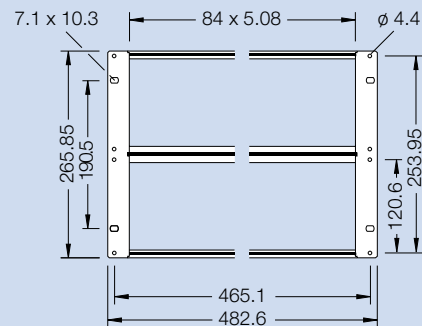
Front of subrack 6 U
